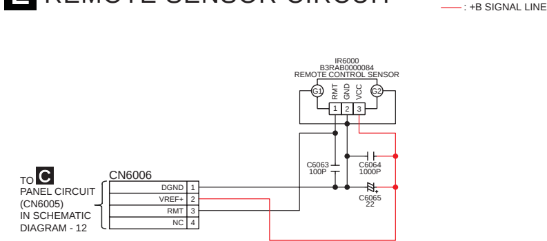
SCHEMATIC DIAGRAM - 14
