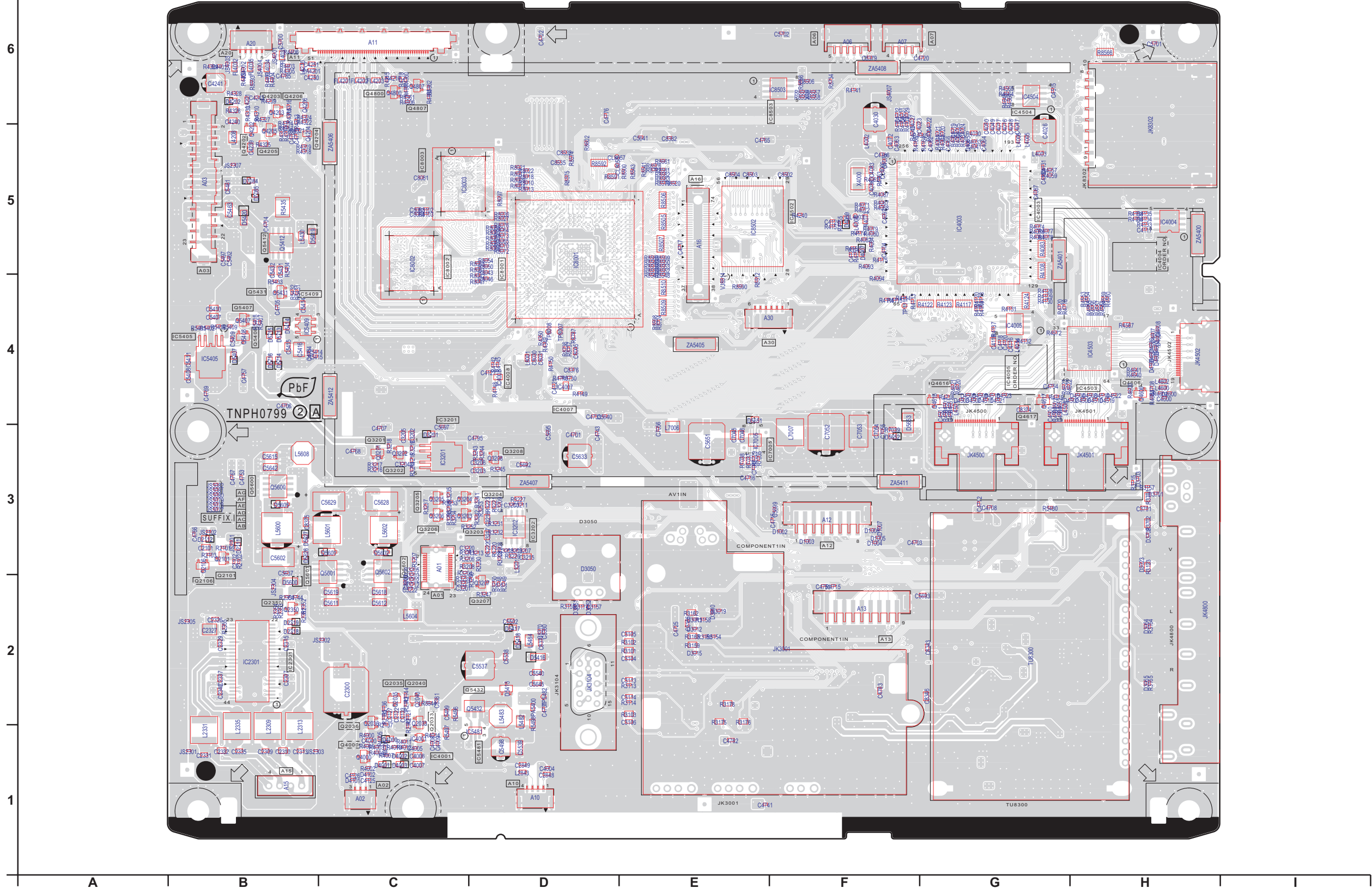
A-BOARD (COMPONENT SIDE) TXN/A10NCSS(32 inch) TXN/A10PTGS(37 inch)
