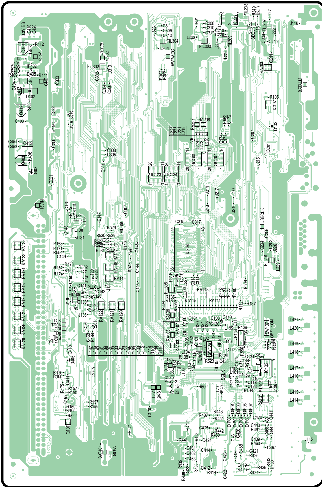
KX-TDA200 MPR CARD BOTTOM VIEW
