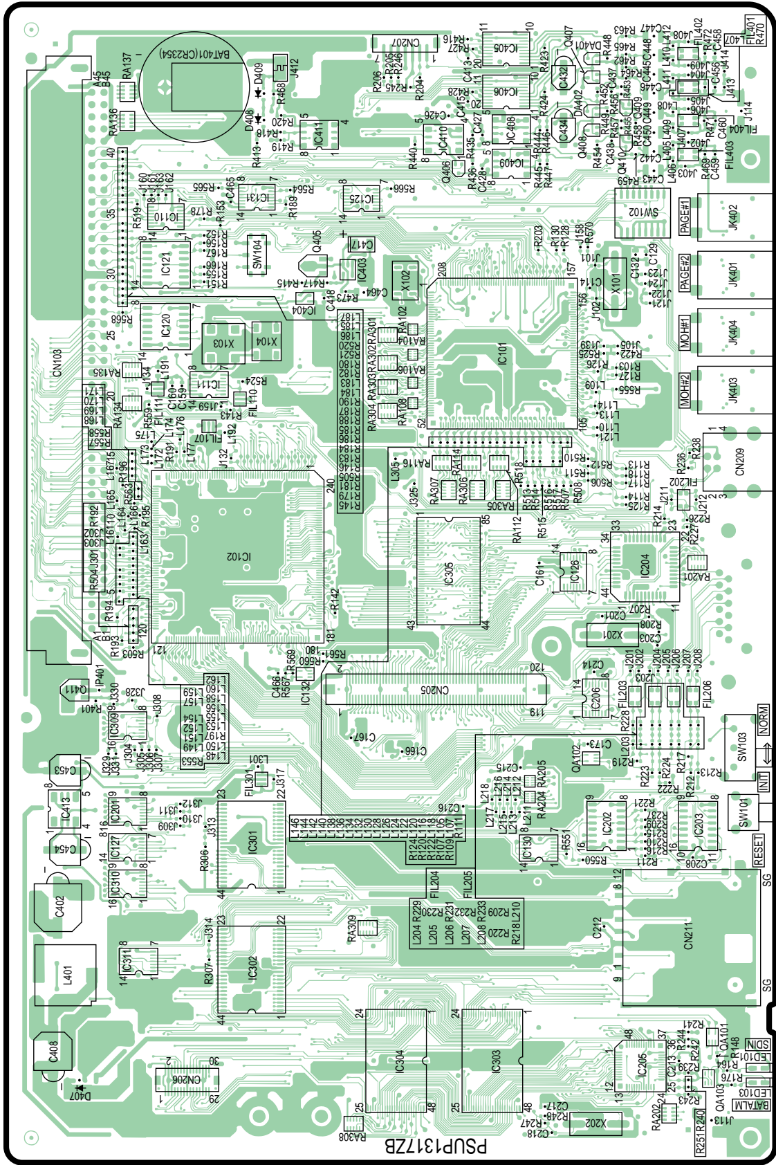
KX-TDA200 MPR CARD COMPONENT VIEW
