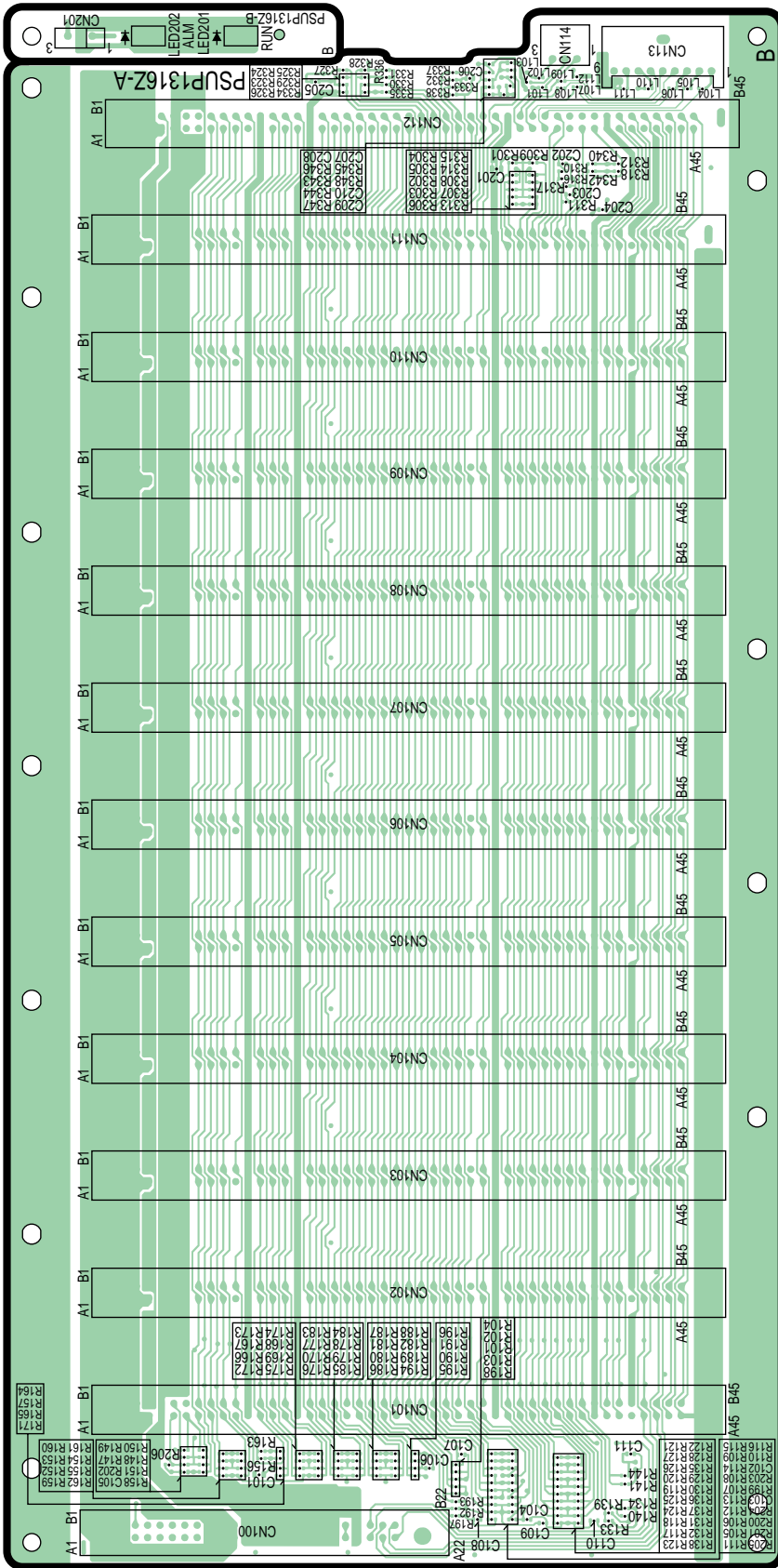
KX-TDA200 BACK/LED BOARD COMPONENT VIEW
