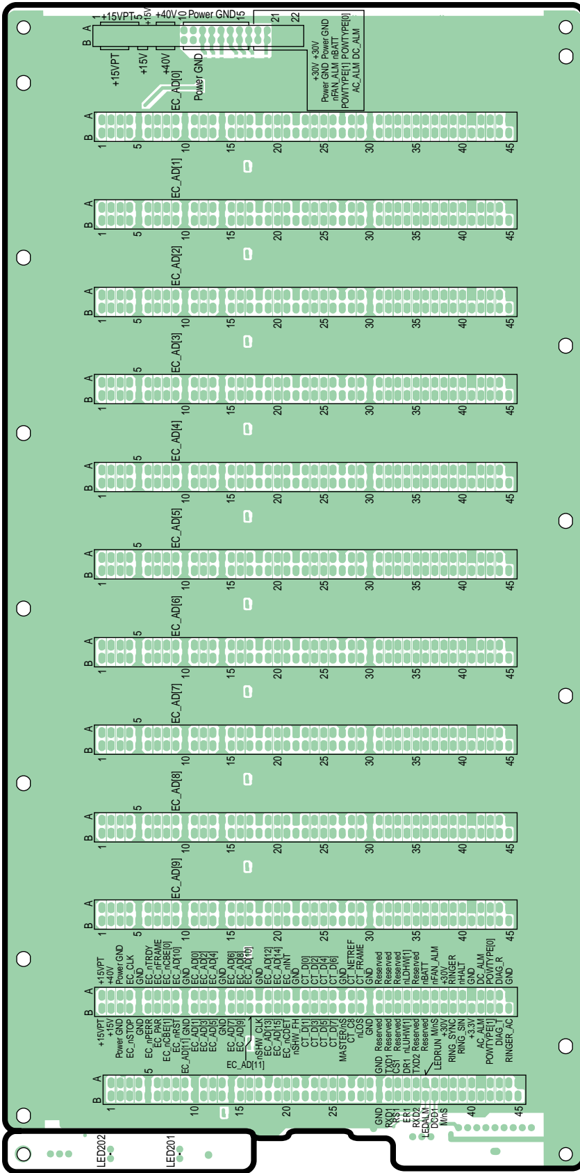
KX-TDA200 BACK/LED BOARD BOTTOM VIEW
